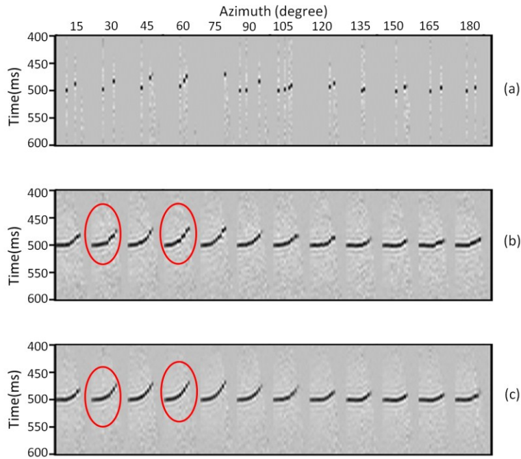
Figure 2: Comparison between different Fourier interpolation methods. (a) Binned input gather for a single CMP. Traces are sorted by azimuth, then offset, for the same azimuth. The azimuth sector spacing is 15 degrees, and the offset bin spacing is 100 m. (b) Interpolated gather using MWNI (Liu and Sacchi, 2004). (c) Interpolated gather using our hybrid 5D method. In the circled area the result of the new method looks more continuous.
