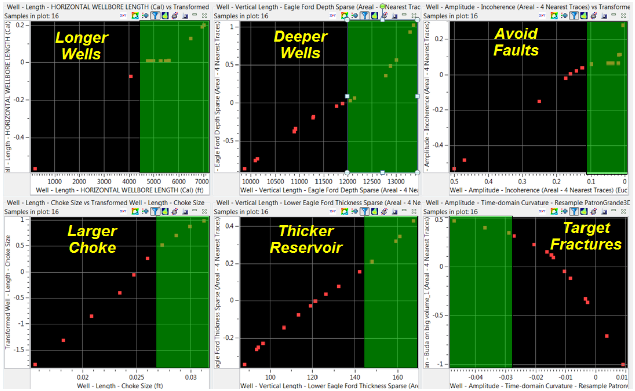
Figure 5: A selection of predictor transformations that highlight (green) the range of parameters and properties that correspond to the greatest well production.
