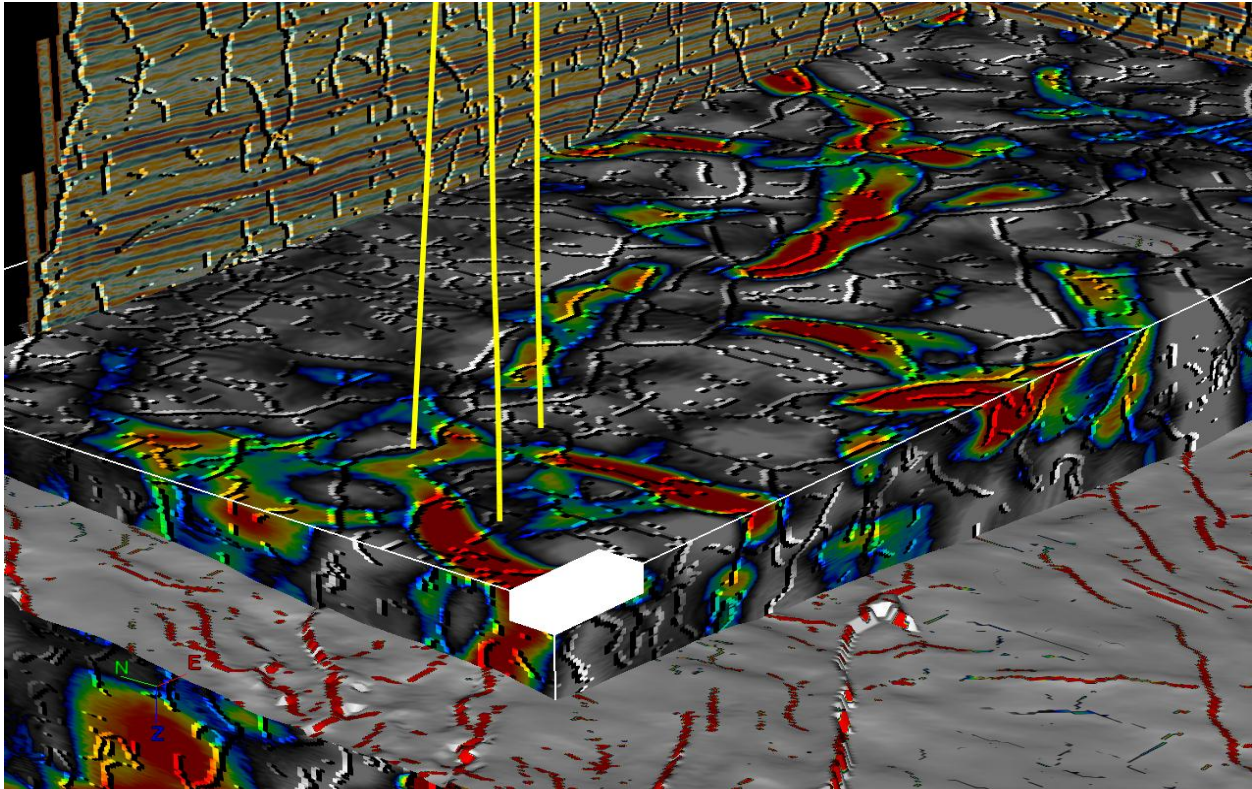
Figure 4: A threshold is set to a fault probability attribute to create a fault proximity volume, where color intensity is an indication of distance to the nearest likely fault. Nearest or average distance to a likely fault is then extracted to each wellbore intersecting the seismic volume.
