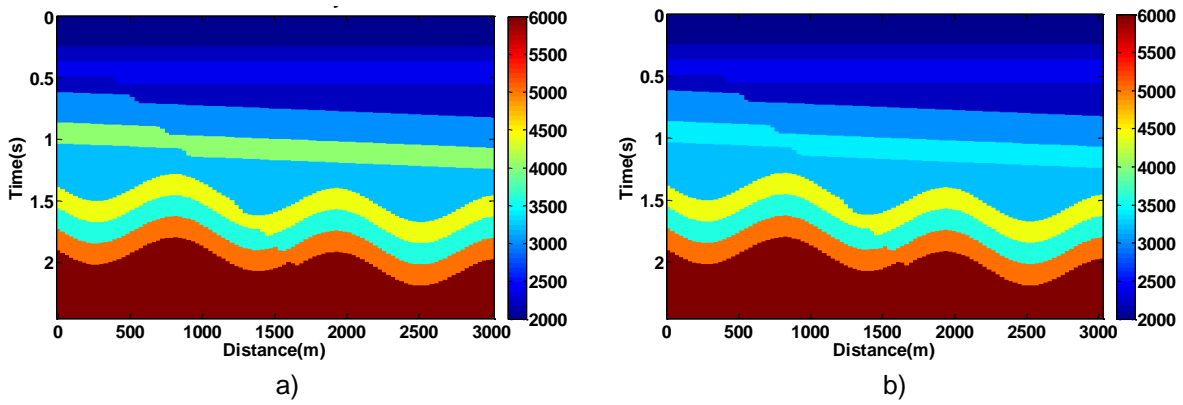
Figure 1: Velocity model for a) baseline, and b) monitor survey.
