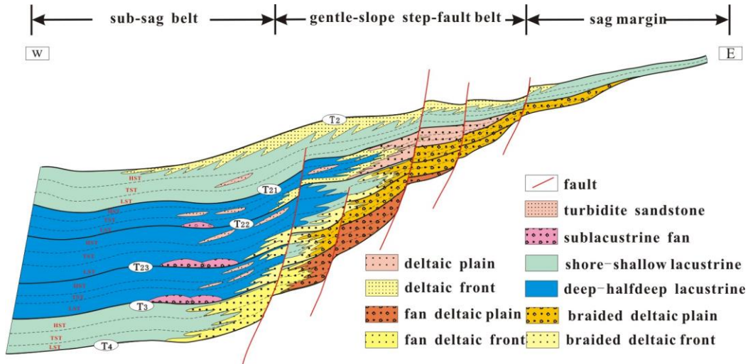
Fig.4. Sequence architecture in the gentle slope of Wuerxun Sag
