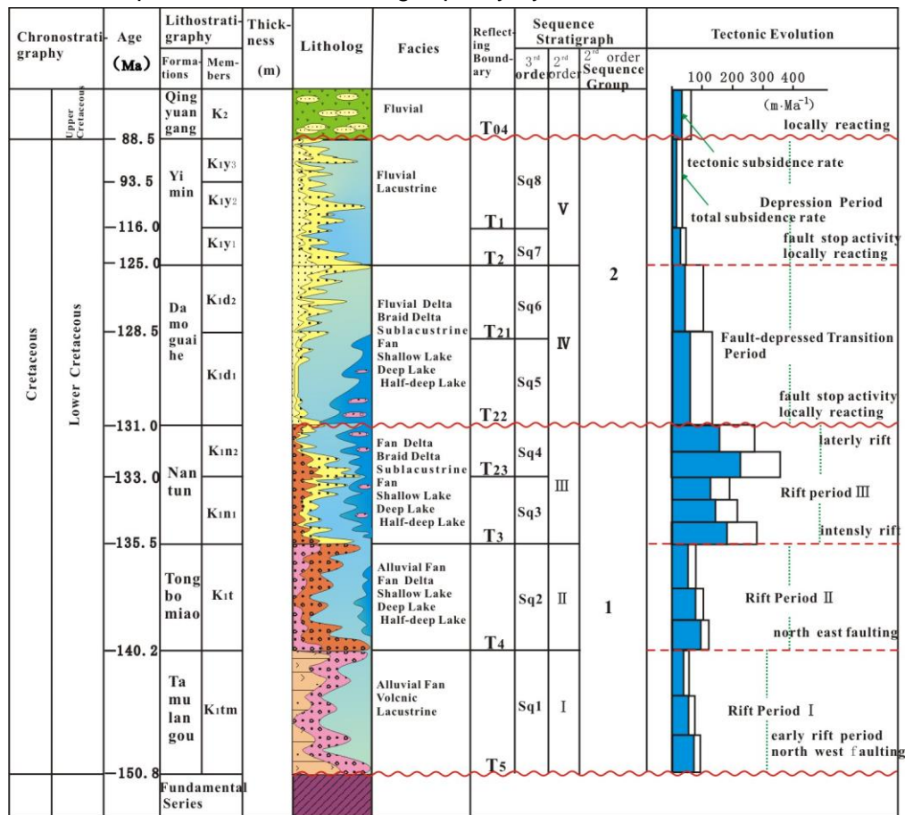
Fig.2. The tectonic evolution of Wuerxun Depression and depositional filling sequences
