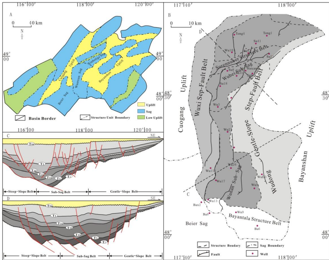
Fig.1. Tectonic lattice frame diagram of Hailar Basin and tectonic lattice frame diagram of Wuerxun Sag
