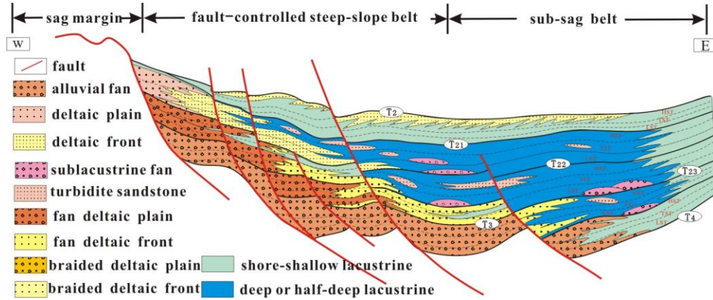
Fig.3. Sequence architecture in the fault-controlled steep-slope belt of Wuerxun Sag
