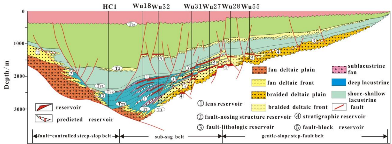
Fig.5. Pattern of oil-gas accumulation in Wuerxun Sag
