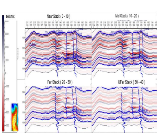
Figure 4: Generation of seismic synthetic models of angle stacks.
