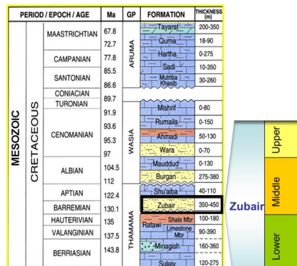
Figure 2: Generalized Kuwait stratigraphic column highlighting Zubair formation.
