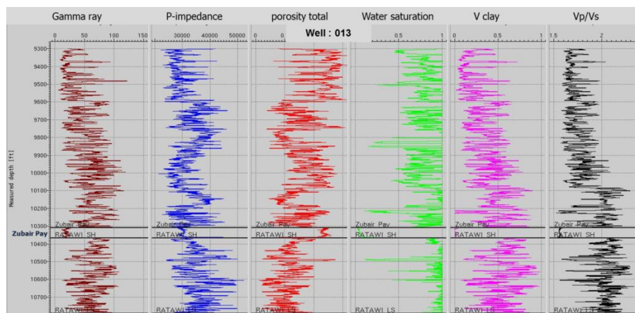
Figure 3: Well log view of Well-013.
