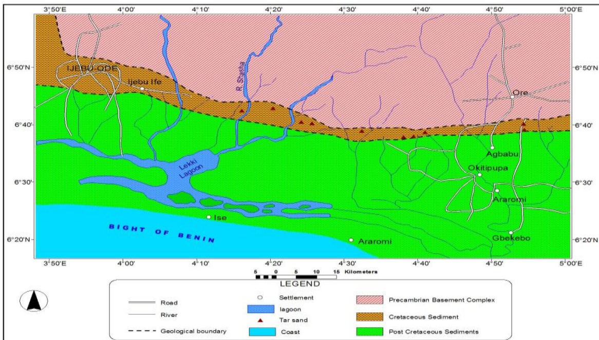
Figure 2: Geology of the Oil Sands belt showing the outcrops ( Adapted from Ako, 2003)
