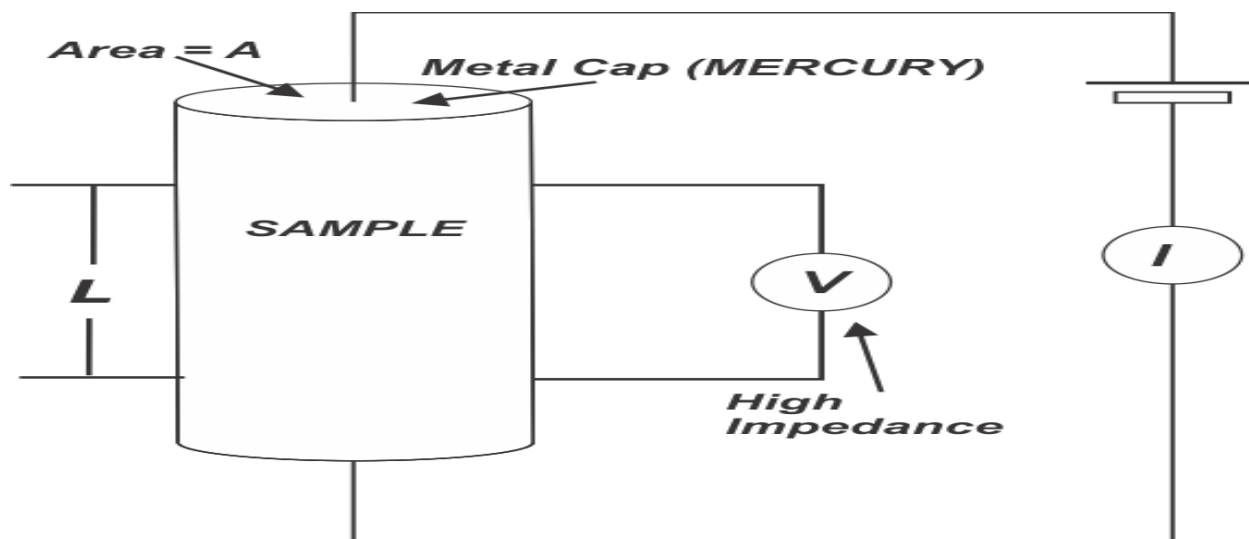
Figure 5: Experimental setup for the determination of Resistivity.
