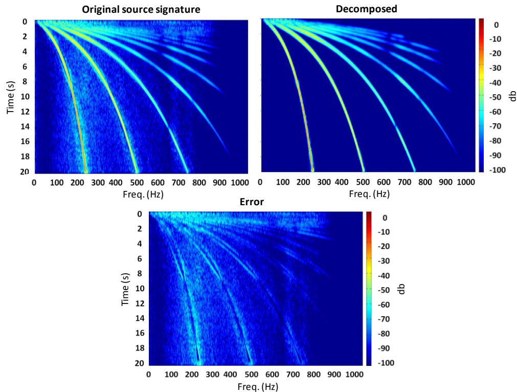
Figure 2: The Gabor spectra for our test source signature (upper left), the final decomposition result (upper right) and the error between the two (bottom).
