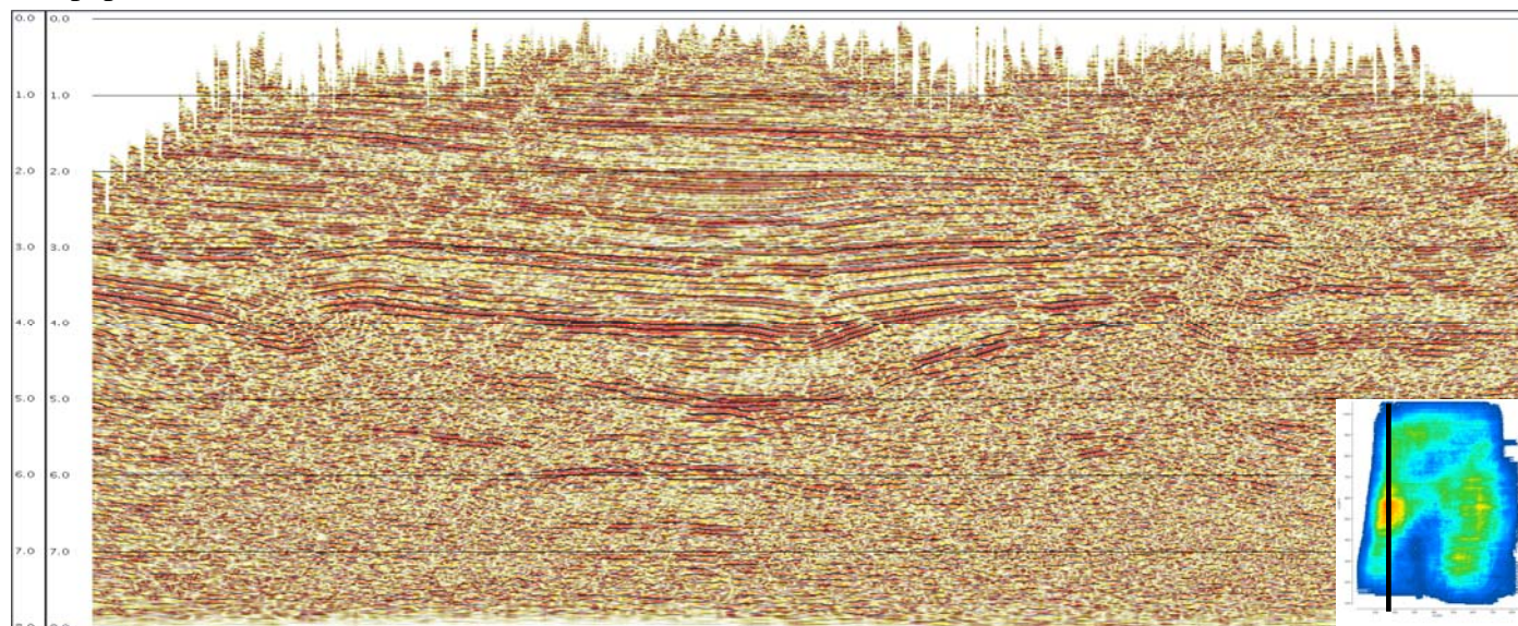
Figure 4: Post-stack QC migration of crossline from the survey. The black line on the inset fold map shows the line location, with the warm colours indicating the higher fold in the centre of the city. The degradation of the data quality on the right corresponds with the lower fold caused by the abandonment of that portion of the survey after the flooding. This is indicated by the blue colours in the South central part of the fold map.
