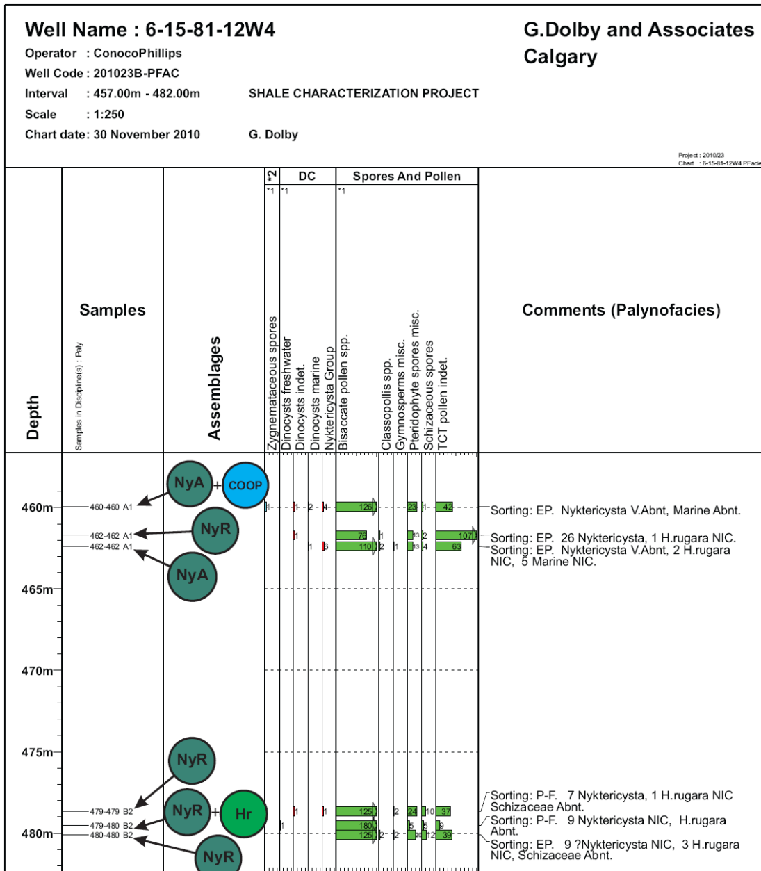
Figure 2. An example of a palynological plot from the 6-15-81-12W4 (Thornbury) well with the COOP designations annotated alongside samples from the B2 and A1 regional flooding shales. Illustrated are Nyktericysta “Rare” and the Hurlandsia rugara fresh to slightly brackish assemblages corresponding to the lower B2 shale, and Nyktericysta “Abundant” and COOP brackish to marginal marine assemblages. Through integration of these palynofloral assemblages with additional sedimentological, stratigraphic and geological data.
