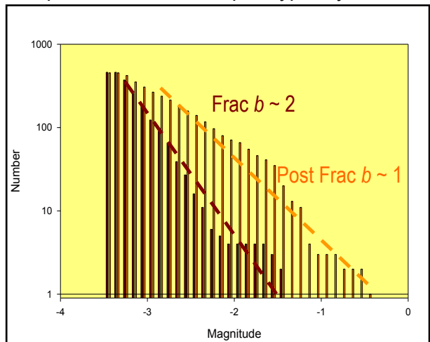
Figure 5. Frequency-magnitude relationship of the microseisms recorded during the frac (red) compared to after the frac (orange).
